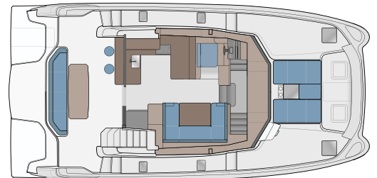
OPTIONAL MAIN DECK W/ INTERIOR HELM
