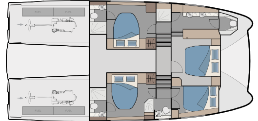
OPTIONAL 4 CABIN + 4 HEAD
