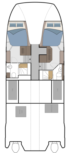
(Outboard Engines)
